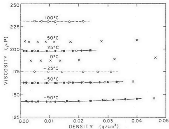
FIG. 2. Viscosity of helium vs density: ●, present results; ○, Flynn, Hanks, Lemaire, and Ross 1 ; ×, Kao and Kobayashi. 3
